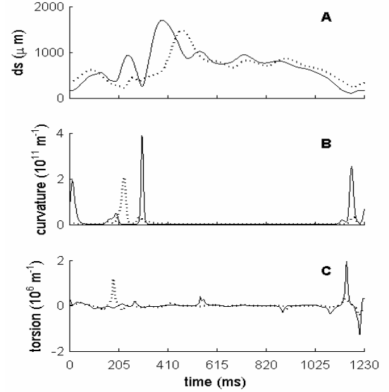
Fig. 3. Scalar parameters characterizing the displacement curve in 3D: (A) displacement (ds), (B) curvature, and (C) torsion within one cardiac cycle at two different phases of the respiration cycle, (FRC) plain line, (FRC+TV) dotted line.
